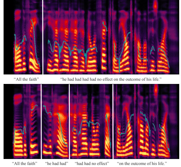
Figure 5: Comparison of Mel spectrograms synthesized by the baseline model (upper part) and the WRF-based model (lower part). The text below the figure corresponds to the transcript. The white line indicates a pause. The green curve represents the F0 trajectory.
